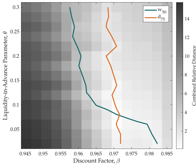
Figure 6: Joint Identification of (\beta, \theta)
